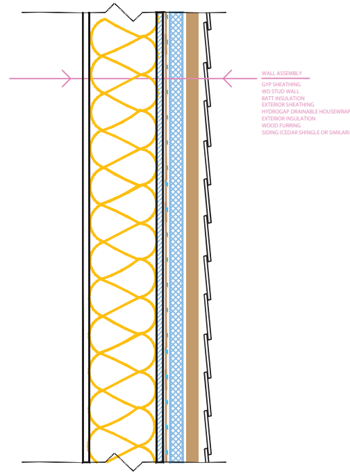
OPTION 2: HYDROGAP SA, EXTERIOR INSULATION, AND WOOD FURRING
