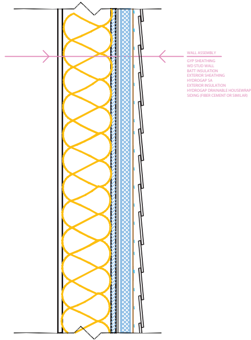
OPTION 1: HYDROGAP SA, EXTERIOR INSULATION, HYDROGAP
