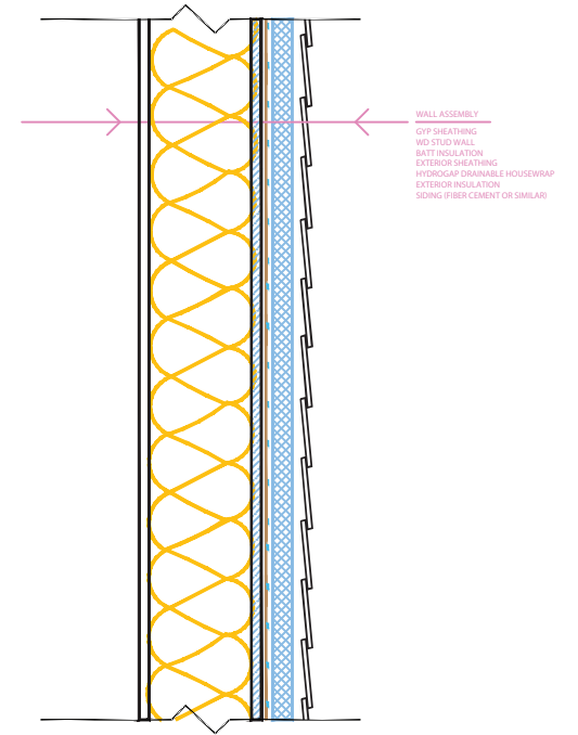
OPTION 3: HYDROGAP SA AND EXTERIOR INSULATION
