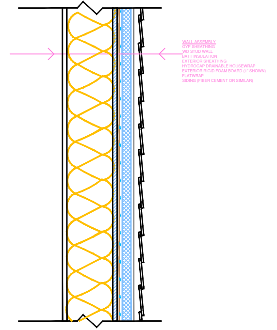
OPTION 3: HYDROGAP, RIGID FOAM AND FLATWRAP
