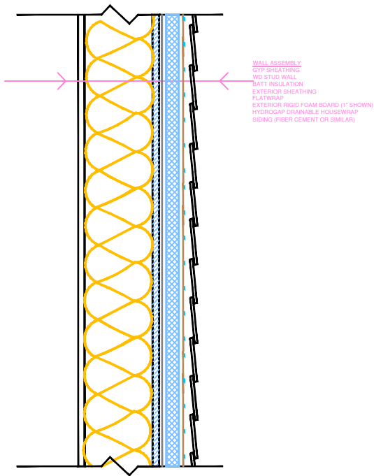
OPTION 1: FLATWRAP, RIGID FOAM AND HYDROGAP
