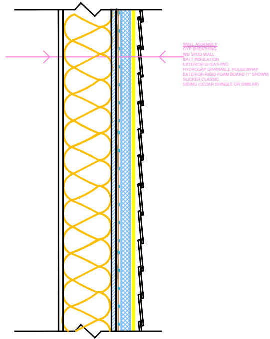
OPTION 2: HYDROGAP, RIGID FOAM, SLICKER CLASSIC
