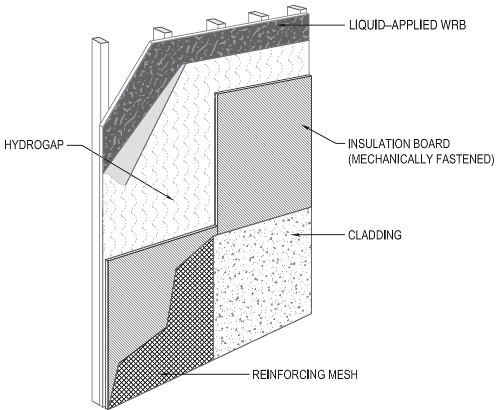
WALL SECTION
