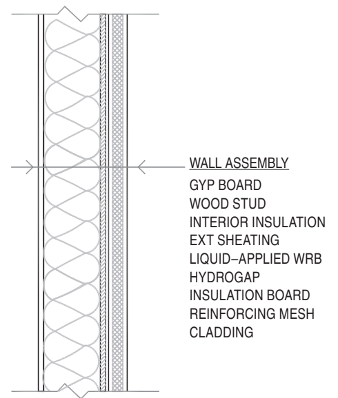
WALL SECTION
