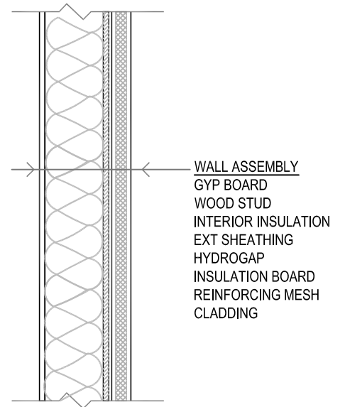
WALL SECTION
