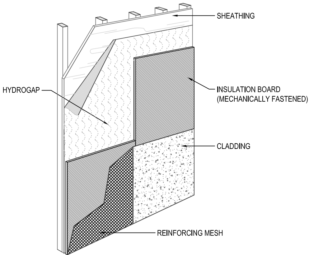
WALL SECTION
